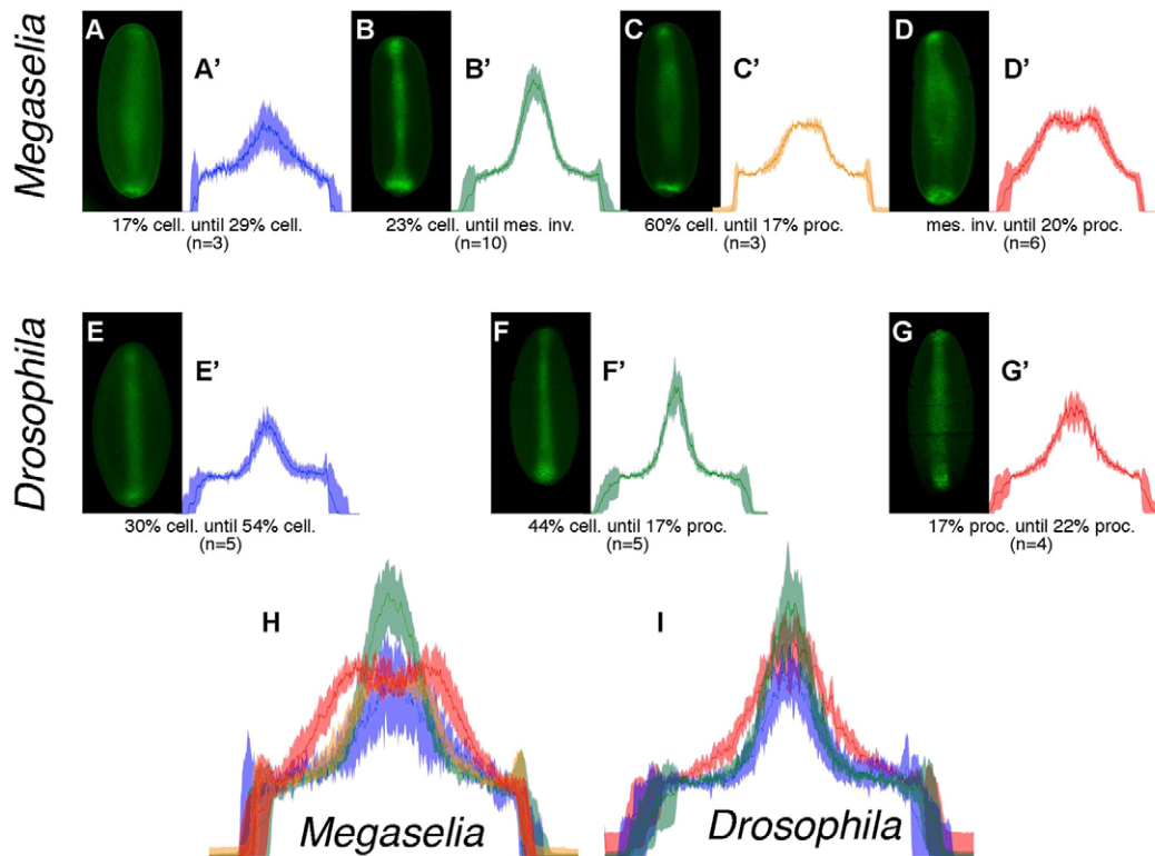
Fig. 5. Distinct pMad dynamics in M. abdita and D. melanogaster .
