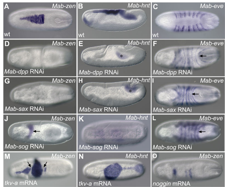
Fig. 9. Representative expression phenotypes following perturbation of BMP signaling. (A-C) Expression of Mab-zen (A), Mab-hnt (B) and Mab-eve (C) in wild-type embryos at early gastrulation stages. (D-L) Expression of the same genes following RNAi against Mab-dpp (D-F), Mab-sax (G-I) or Mab-sog (J-L). Proctodeal expression of Mab-hnt (asterisks in E,H), circumferential Mab-eve stripes (arrows in F,I,L), and the broadened residual expression domain of Mab-zen (arrow in J) are indicated. (M,N) Expression of Mab-zen (M) or Mab-hnt (N) following injection of tkv-a mRNA. Note the repression of endogenous expression near ectopically induced expression (arrows in M). (O) Expression of Mab-zen following injection of Xenopus noggin mRNA. Anterior is to the left in dorsal (A,C,D,F,G,I-O) or lateral (B,E,H) view.
