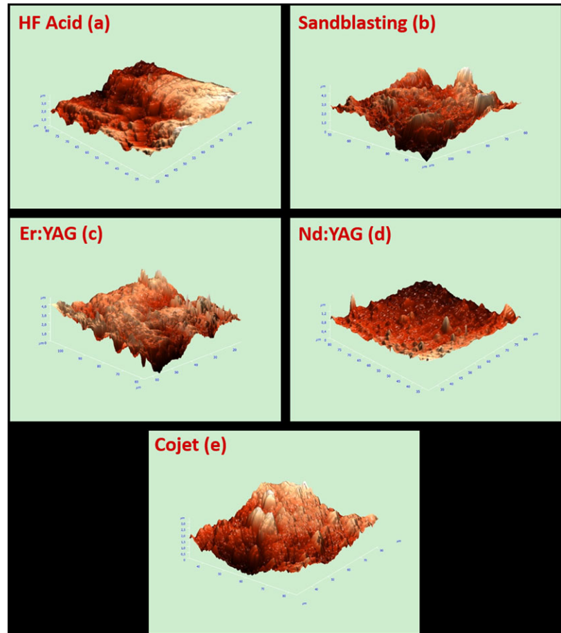
Figure 3 Atomic force micrographs of Vita In-Ceram zirconia specimens subjected to different surface treatments.
