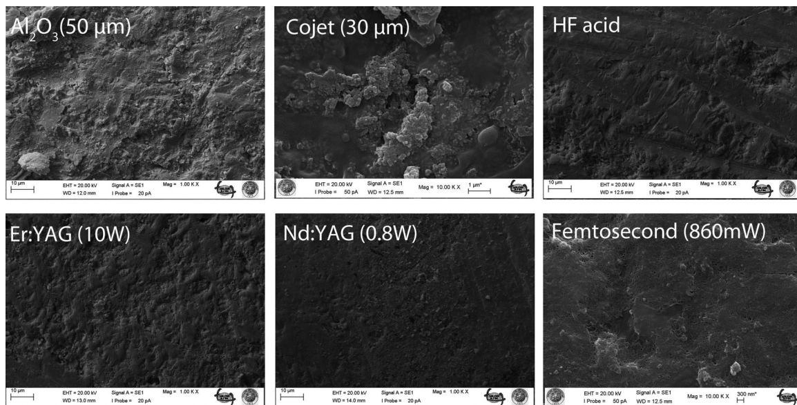
Figure 5 Scanning electron micrographs of Vita In-Ceram zirconia specimens subjected to different surface treatments.
