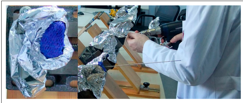
Figure 3. (Left) Scapula model covered by aluminum foil, mounted on the fixture, (Right) Experiment setup, surgeon inserting the guide pin with the freehand method.
