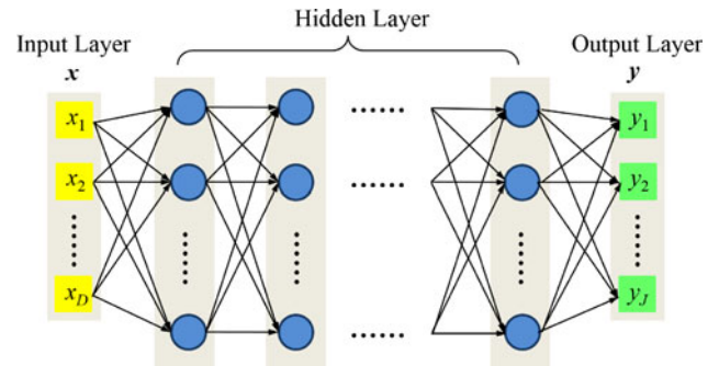
Fig. 2. Structure of a DNN model.
