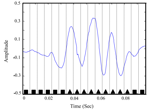
Fig. 6. A K-means clustering result using 39 MFCC with Euclidian distance on an S1 heart sound segment.
