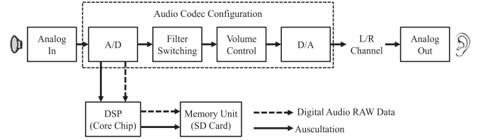
Fig. 3. Block diagram for the electronic stethoscope used in study.
