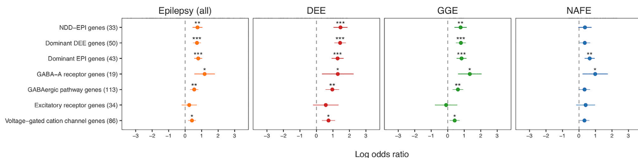
Figure 2. Burden of Ultra-Rare Singletons Annotated as Protein-Truncating Variants or Damaging Missense (MPC \geq 2) Variants “Ultra-rare” variants (URVs) were defined as not observed in the DiscovEHR database. Gene sets were defined in Table S6 and the number of genes was specified in the parenthesis. DEE stands for individuals with developmental and epileptic encephalopathies, GGE for genetic generalized epilepsy, NAFE for non-acquired focal epilepsy, and EPI for all epilepsy; NDD-EPI genes are genes with de novo burden in neurodevelopmental disorders with epilepsy. Asterisks indicate significance after FDR control (* for FDR-adjusted p value < 0.05 , ** for adjusted p value < 1 \times 10^{-3} , and *** for adjusted p value < 1 \times 10^{-5} ). Effects were displayed in odds ratios with the corresponding 95% confidence intervals (CIs).
