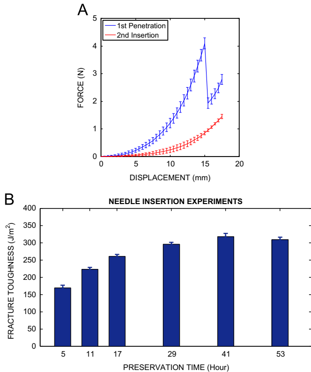
Fig. 7 – (A) The force displacement responses of the bovine liver of Animal #1 during the first and second needle insertions. (B) The change in fracture toughness of bovine liver (average of three animals) as a function of preservation time.
