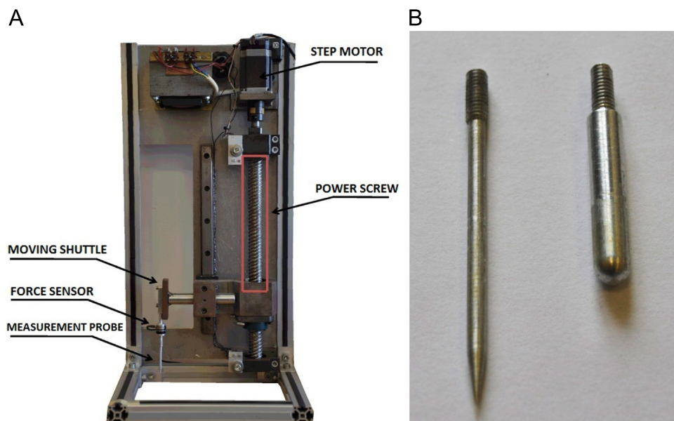
Fig. 2 – (A) Our set-up for conducting mechanical characterization experiments. (B) The needle (diameter=3 mm) and the cylindrical probe (diameter=6 mm) used for the mechanical characterization experiments.
