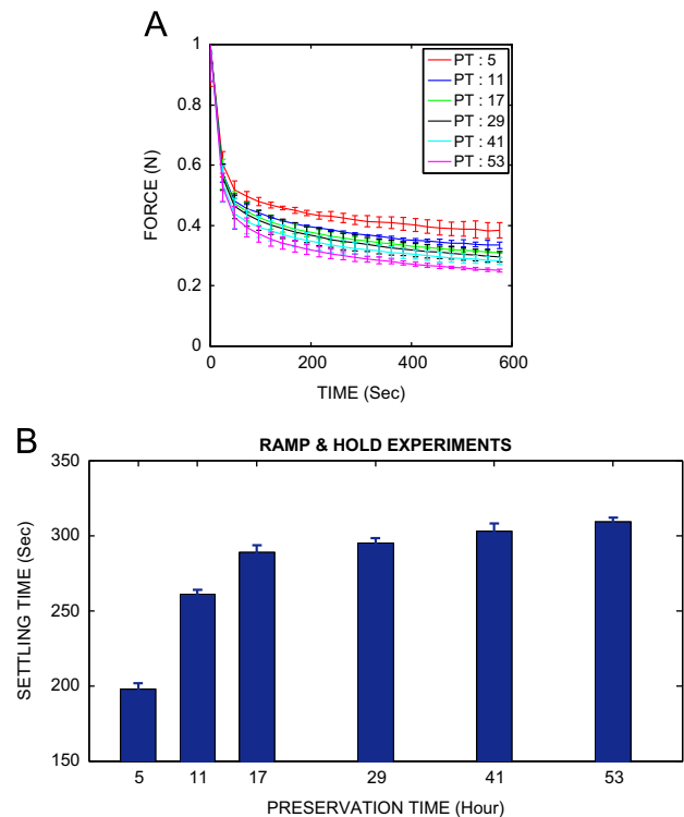
Fig. 6 – (A) The normalized force relaxation response of bovine liver (average of three animals) for different preservation times. (B) The settling time of the relaxation response for different preservation times.
