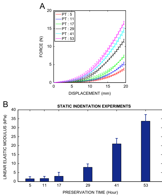
Fig. 5 – (A) The force response of bovine liver (average of three animals) as a function of compression depth for different preservation times. (B) The linear elastic modulus of bovine liver (average of three animals) as a function of preservation time.
