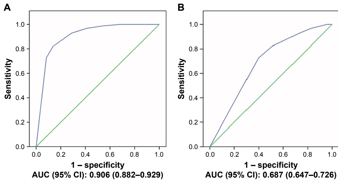
Figure 1 Receiver operating characteristic curve (ROC) analysis of the MNA-SF to detect (A) frailty and (B) pre-frailty.
