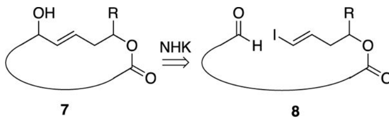
Figure 2. General approach to macrocyclic allylic alcohols.
