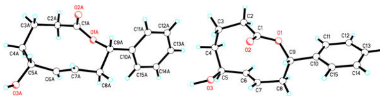
Figure 4. X-ray crystal structures for 21a (left) and 21b (right).
