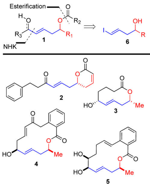
Figure 1. Design rationale for structures of natural products containing hydroxy vinyl core (1): rugulactone (2), aspinolide A (3), pochonin F (4), and aigialomycin D (5).
