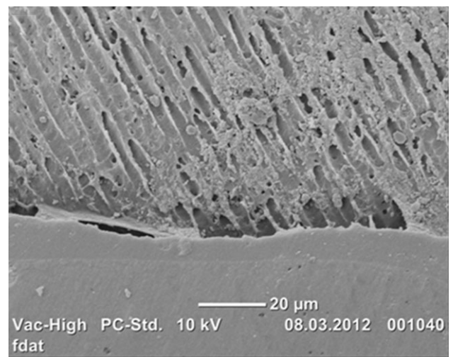
FIGURE 15. Scanning electron microscope image of dentin–G-Aenial Bond interface of two consecutive coats groups.
