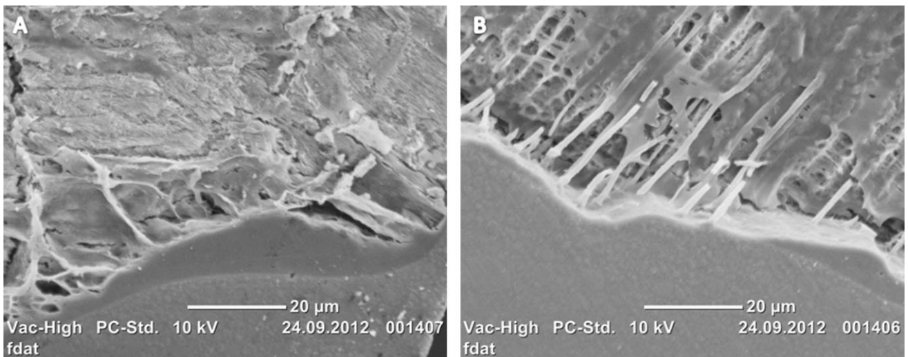
FIGURE 12. Scanning electron microscope image of A, enamel–G-Aenial Bond and B, dentin–G-Aenial Bond interface of control groups.
