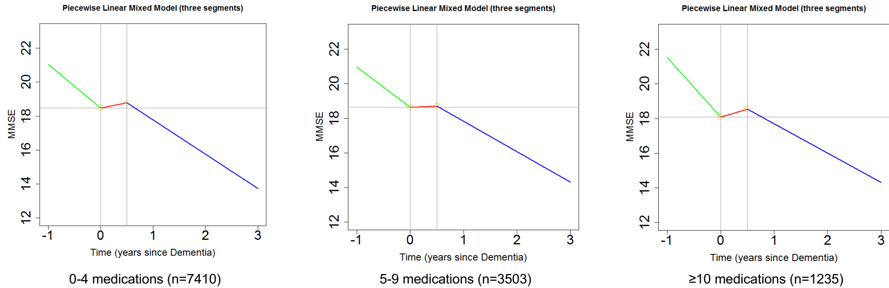
Figure 2: Comparison of non-parametric Linear Mixed Models of the rate of cognitive decline allowing adjustment for co-variates
